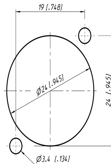
Panel cut outy (rear side)
