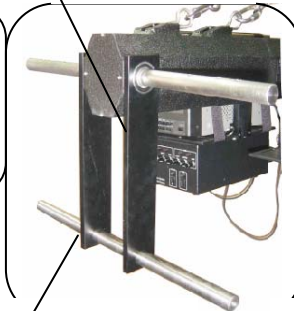
Counterweight rod
