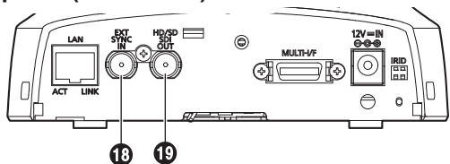
<Rear panel (AW-HE60S)>
