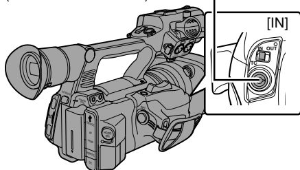
Slave Device (This Camera Recorder)
