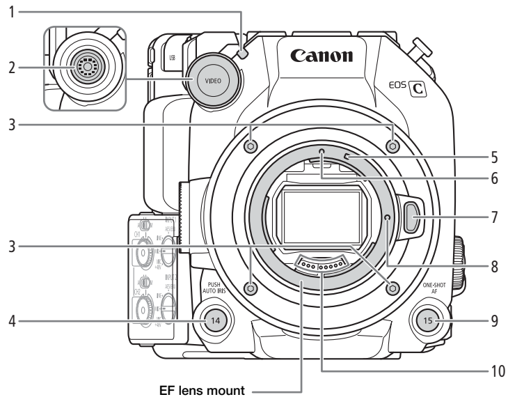
EF lens mount
