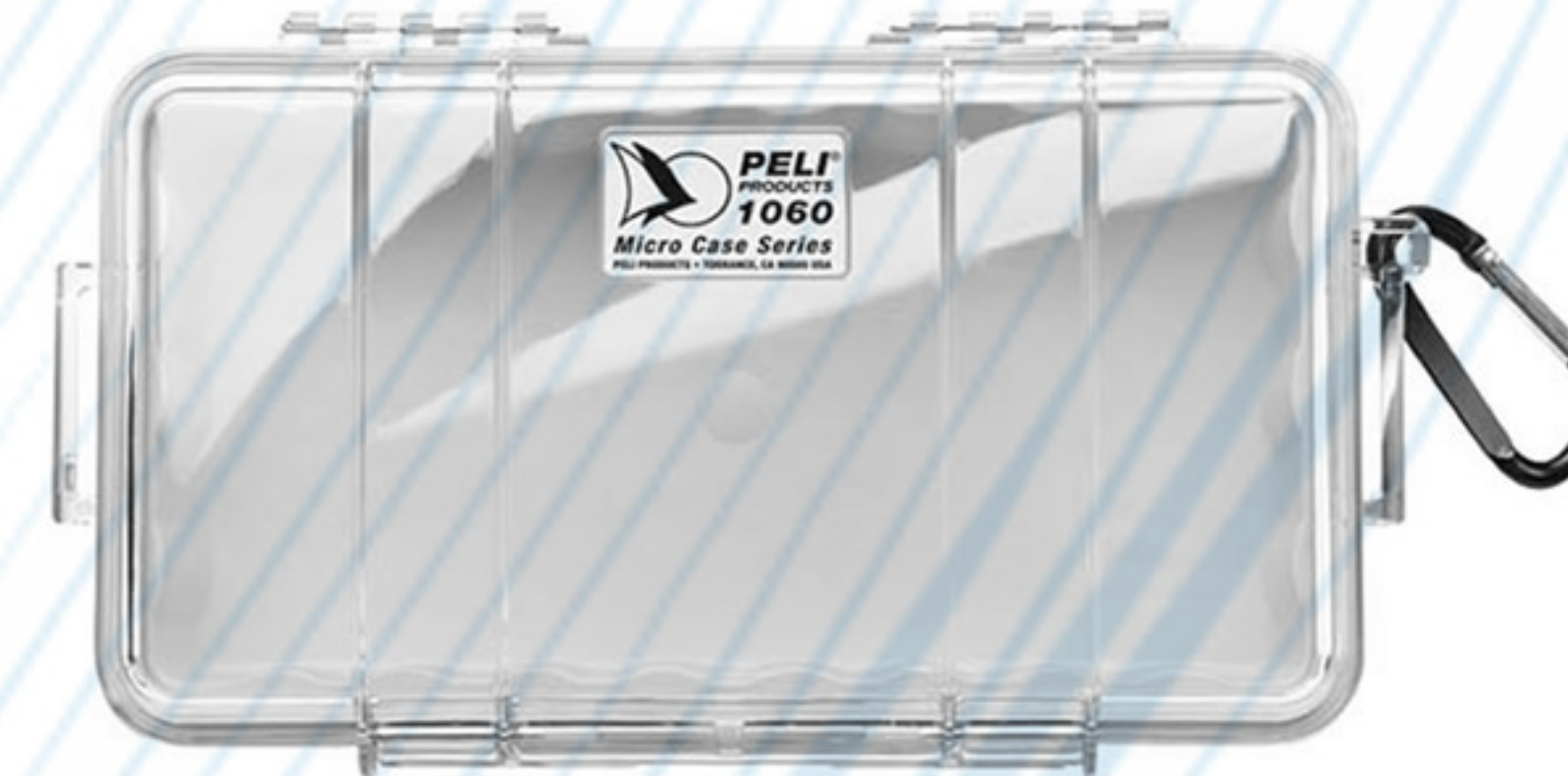
1060-Clear-Yellow 1060-Micro-Case-Clear-Yellow (1060-025-100E) Interior(WxHxD): 210x58x110mm
